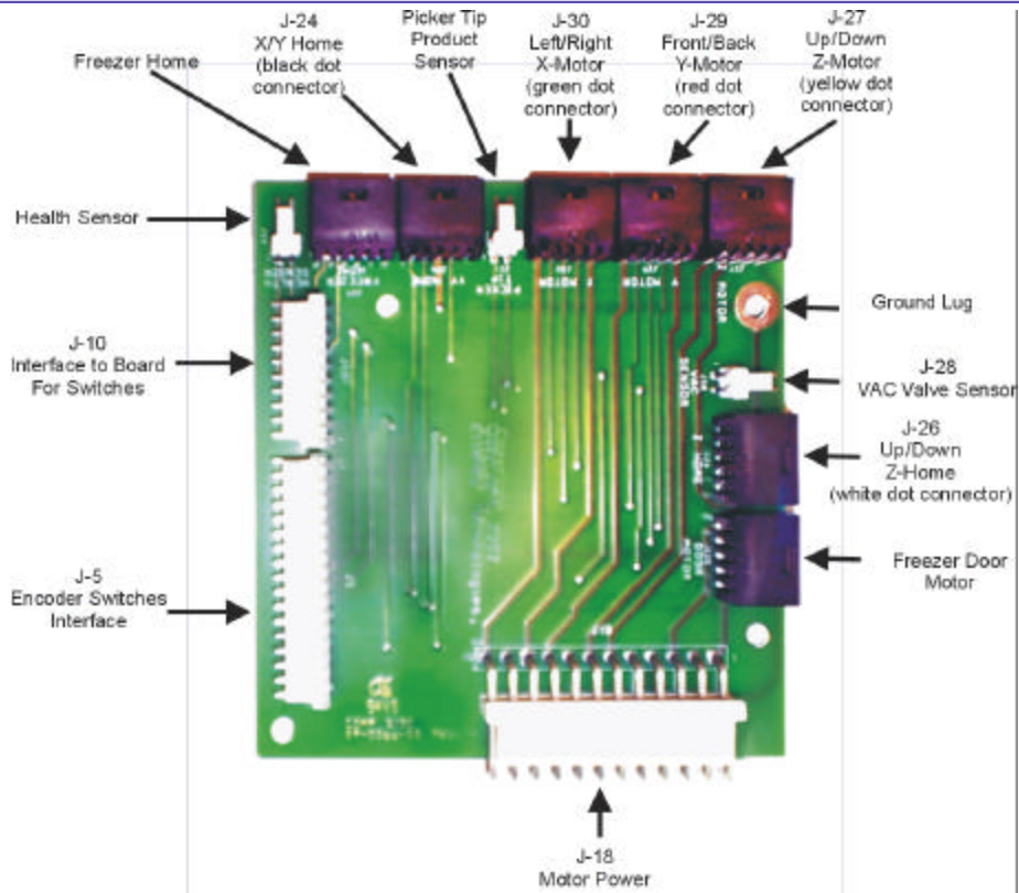
Fig. 5 (Cable Interface Board)
