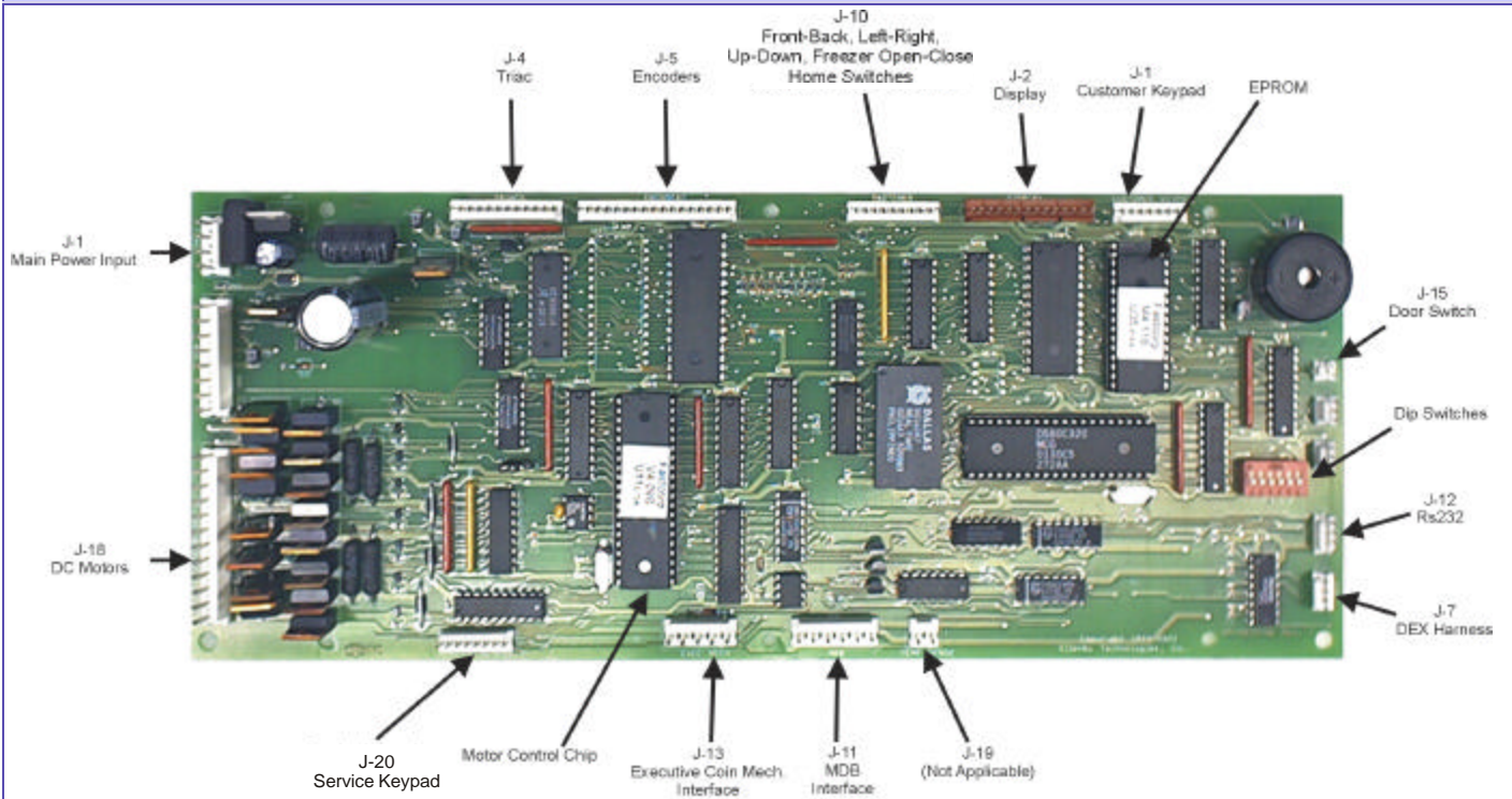
Fig. 4 (Computer Board)
