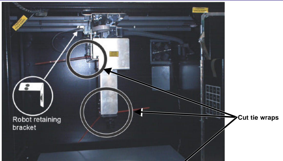
Fig. 17 (Robot Retaining Bracket & Shipping Tie Wrap Locations)
