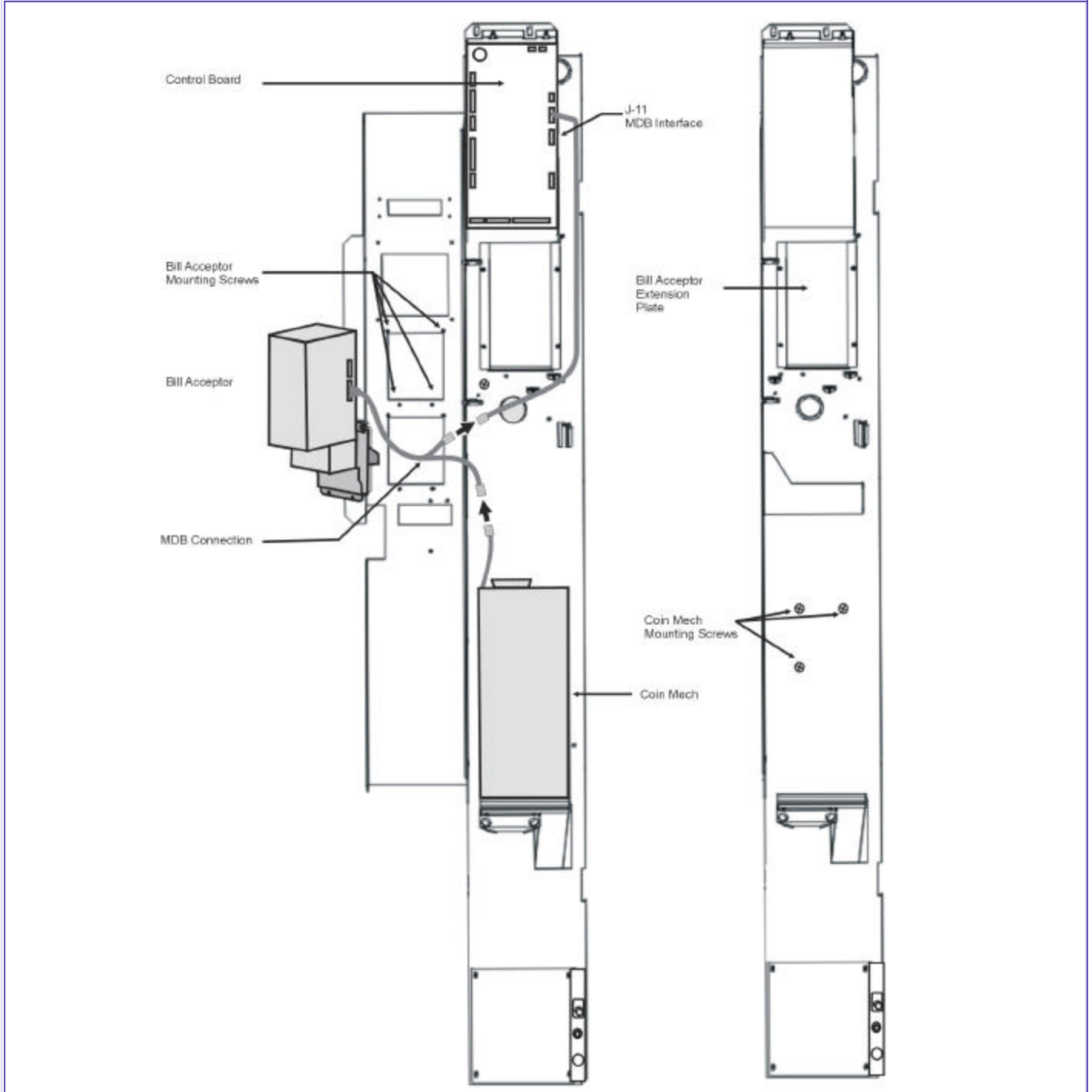
Fig. 18 (Multi-Drop Bus (MDB) Money System Connections and Installation)
