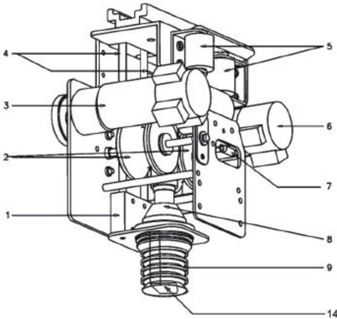
Fig. 13 (Robot Carriage Front/Right)
